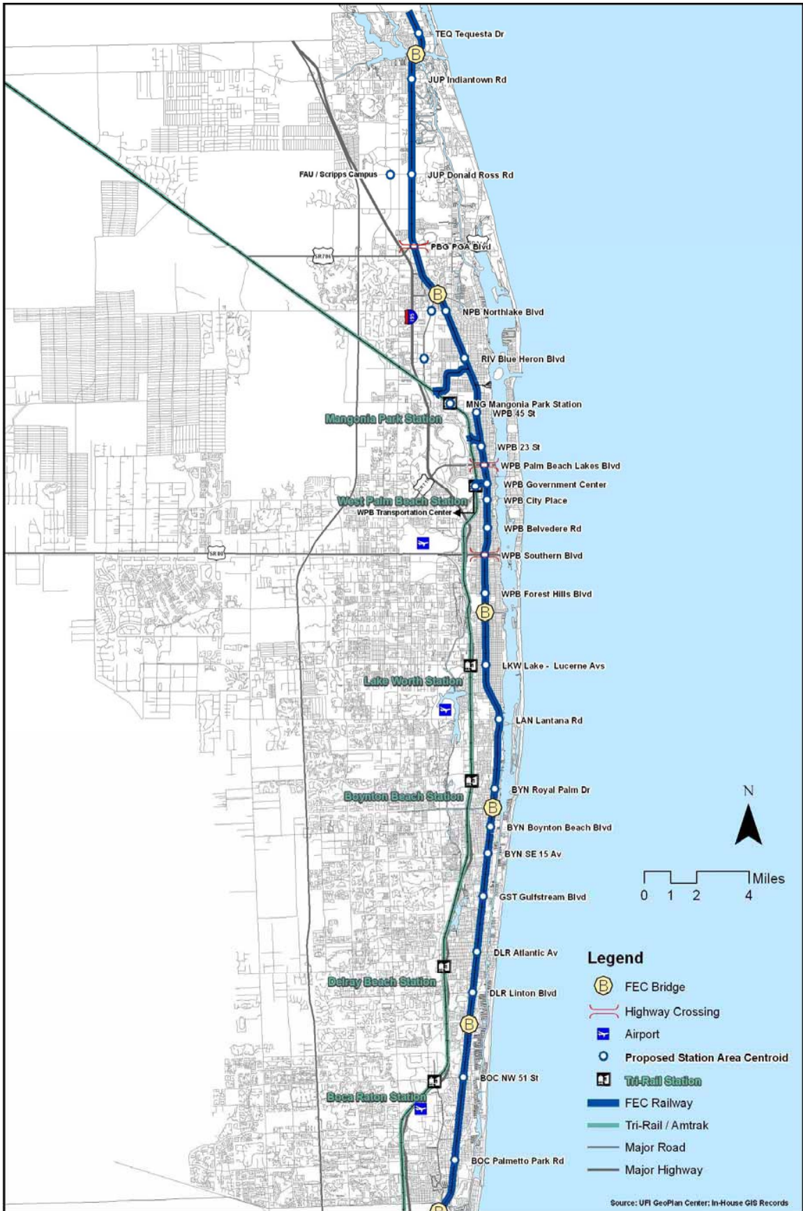
Figure J.9 SFECC Bridges and Highway Crossings (Palm Beach County)
